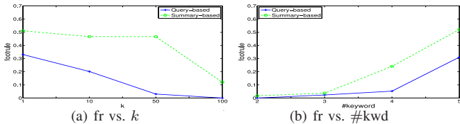
Fig. 4. Footrule vs. k and #kwd
